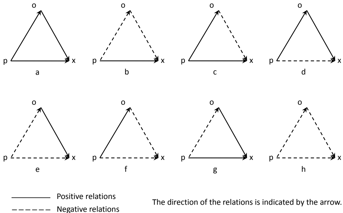
Figure 1: Balanced and unbalanced cognitive triads. Triads a, b, e and f are balanced states; triads c, d, g and h represent unbalanced states.
